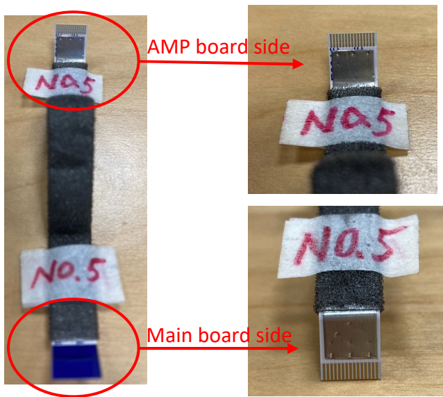
Combined thermal cycling test sample
